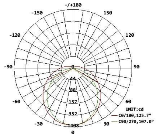
AVERAGE BEAM ANGLE(50%):116.4 DEG A00-530WT-G5-T
